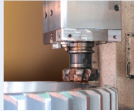
Face milling
