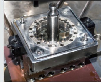
Couvic Coupling type Tool Holder
